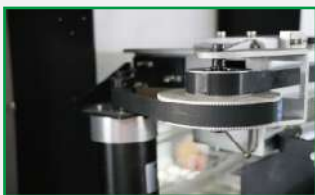
High-precision and high-stability tensioning pulley system.
